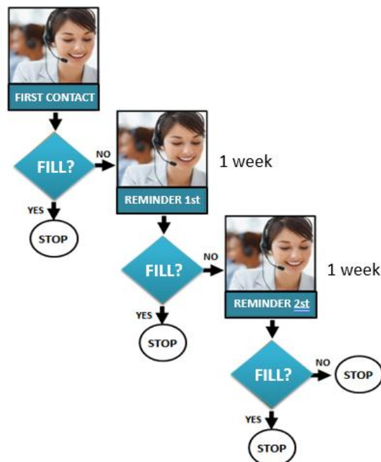
Gambar 3.4 Prosedur Reminder
